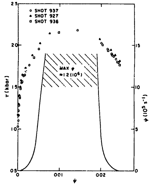
FIG. 5. Plastic-flow process for three shocks at 37 kbar.
